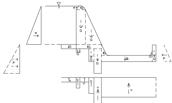
Gambar 2. sketsa tekanan uplift
